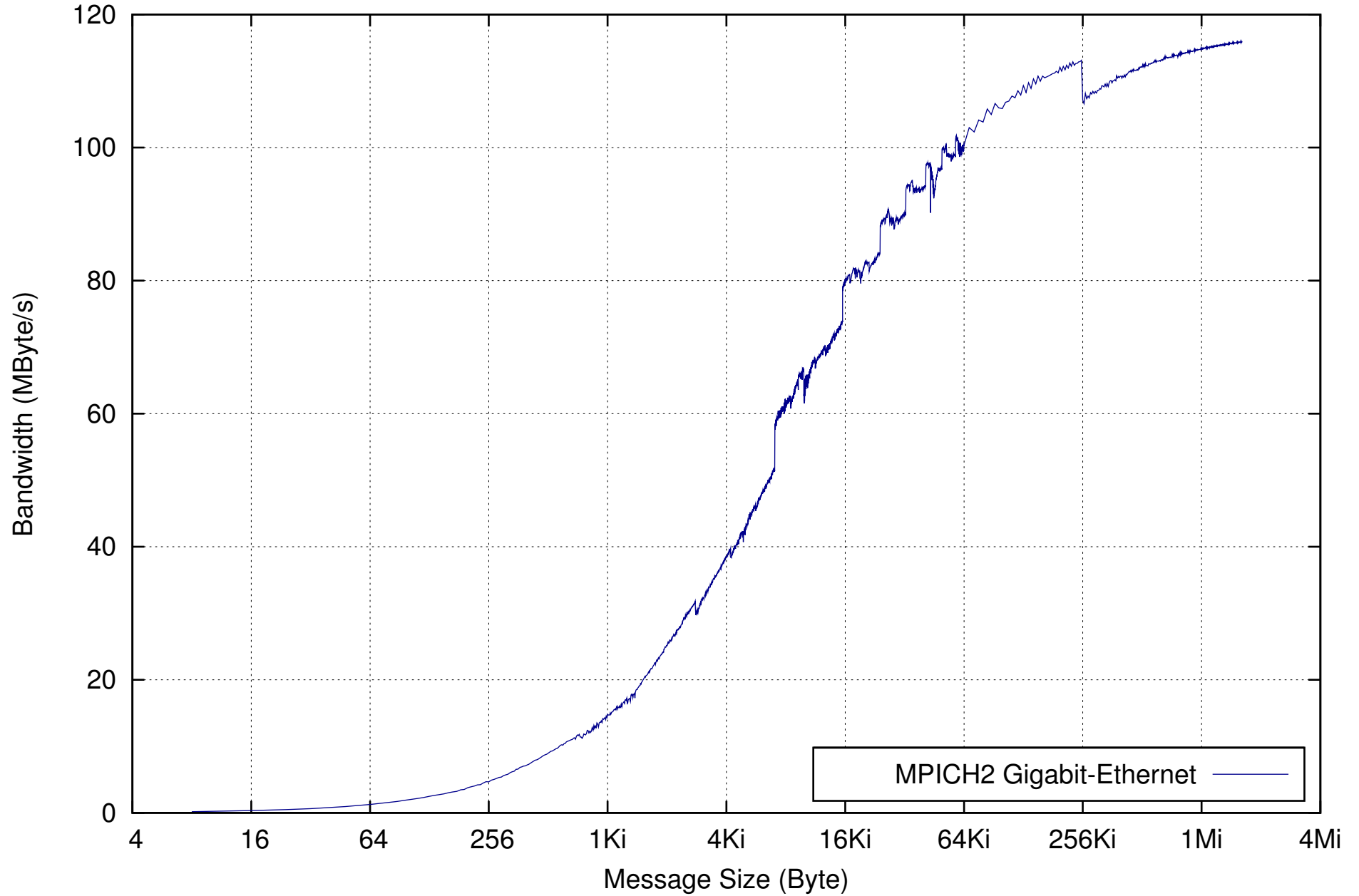
Bandwidth Zuse-Cluster, MPICH2 with MPD via Gigabit-Ethernet
