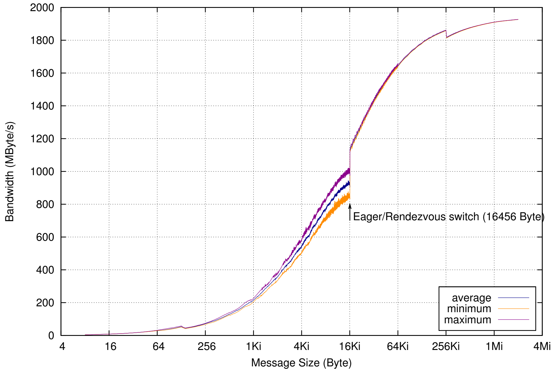
Bandwidth fluctuations Zuse Cluster, Intel MPI over IB
