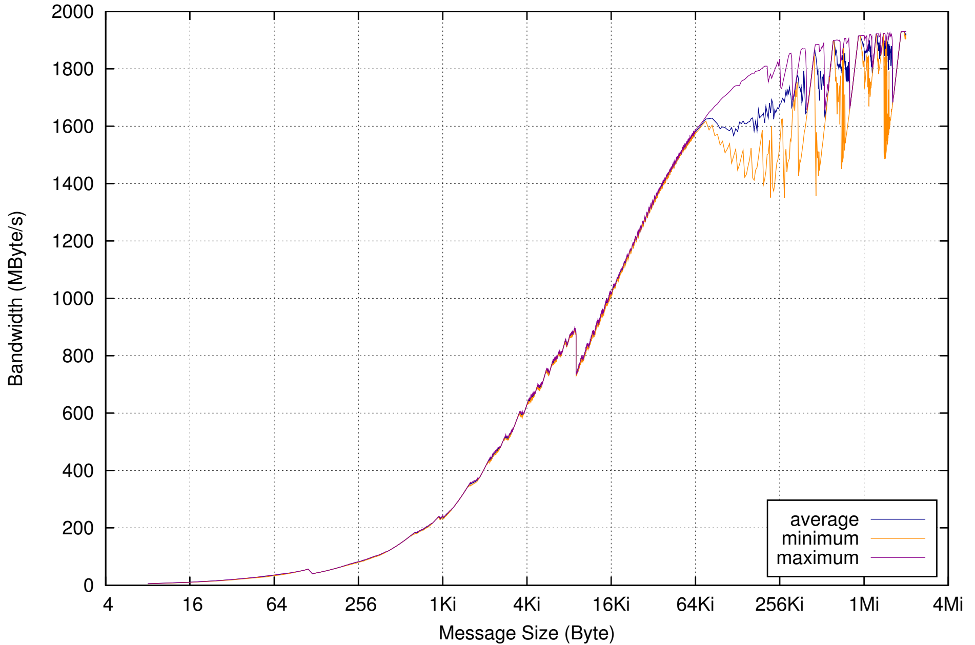
Bandwidth fluctuations Zuse Cluster, MVAPICH/gcc over IB
