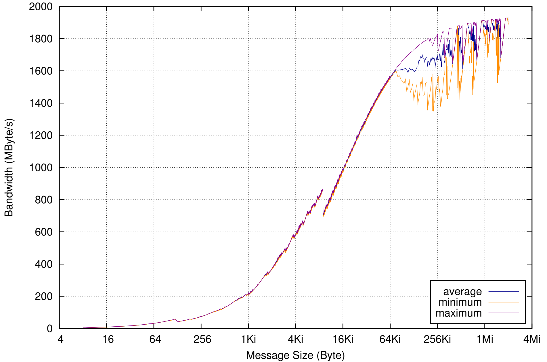
Bandwidth fluctuations Zuse Cluster, MVAPICH2/gcc over IB
