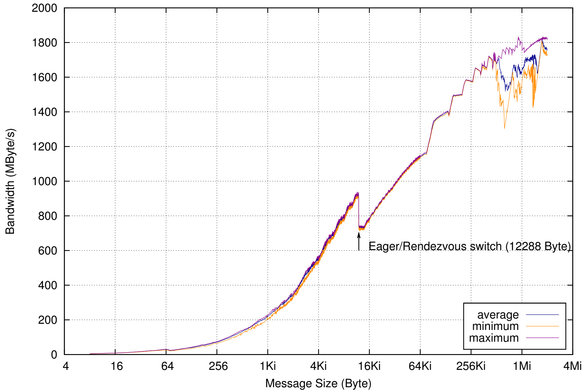
Bandwidth fluctuations Zuse Cluster, Open MPI with gcc over IB
