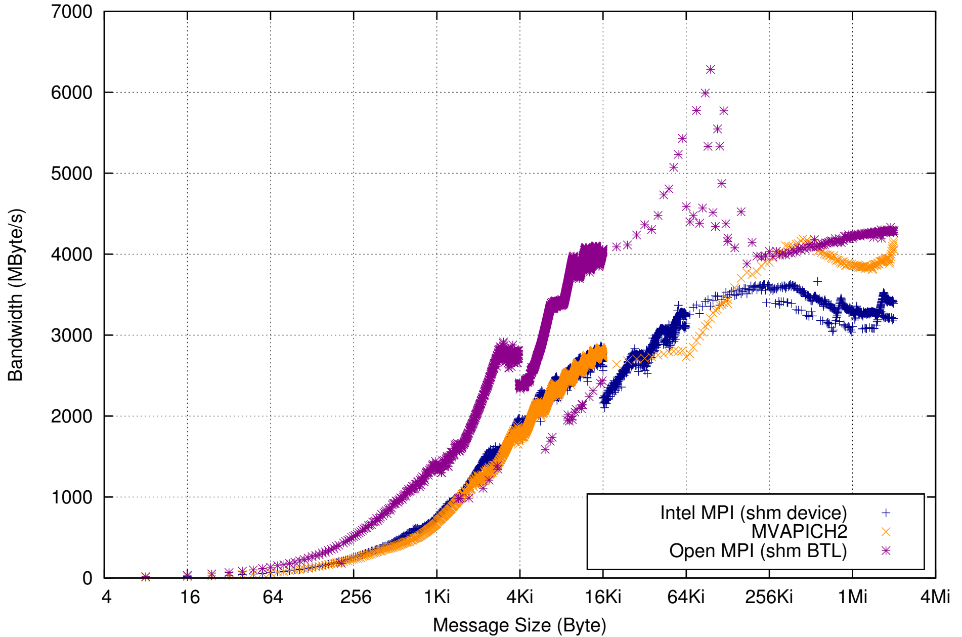
Intra Node communication Zuse Cluster, bandwidth comparison
