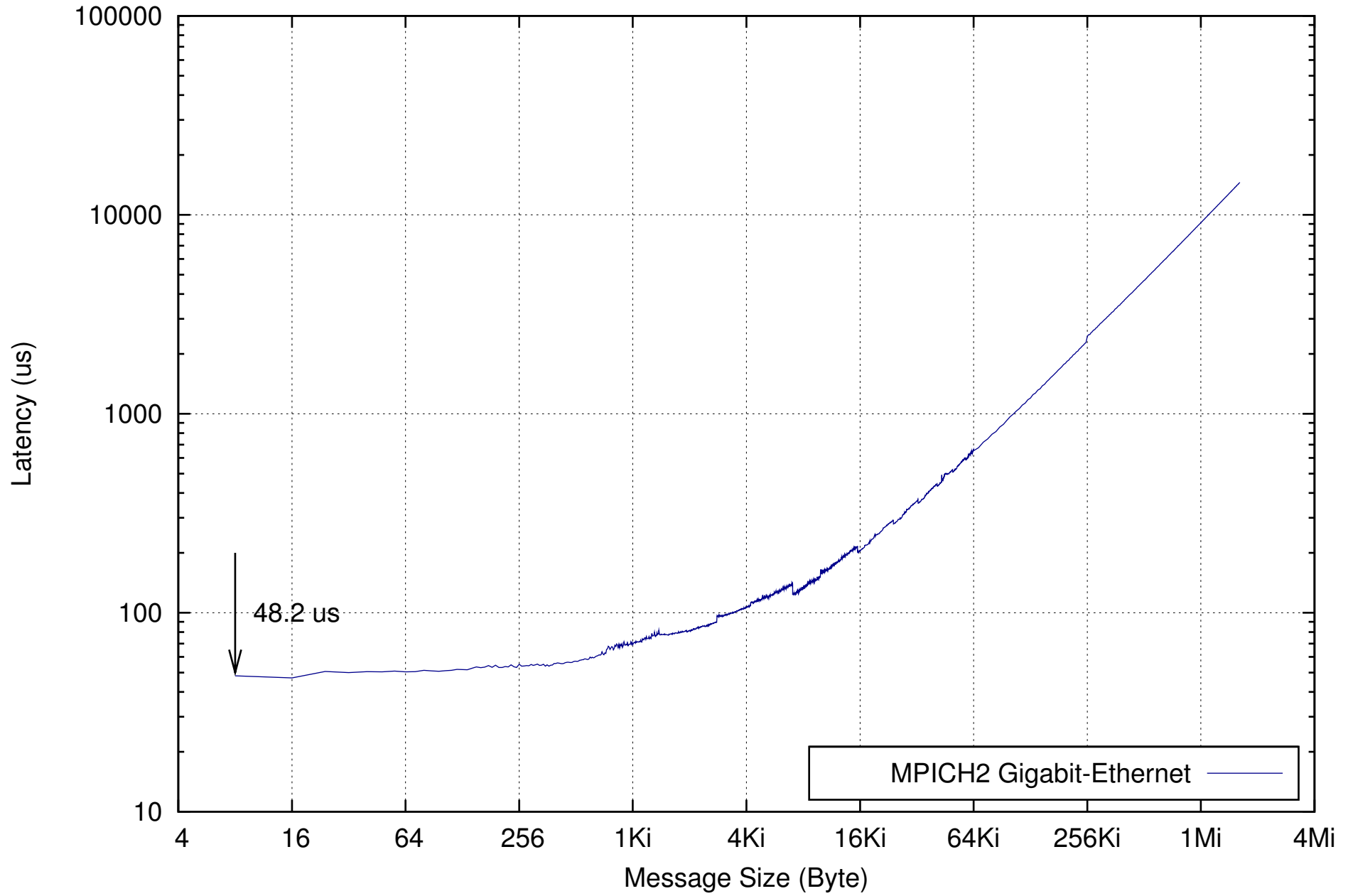
Latency Zuse-Cluster, MPICH2 with MPD via Gigabit-Ethernet
