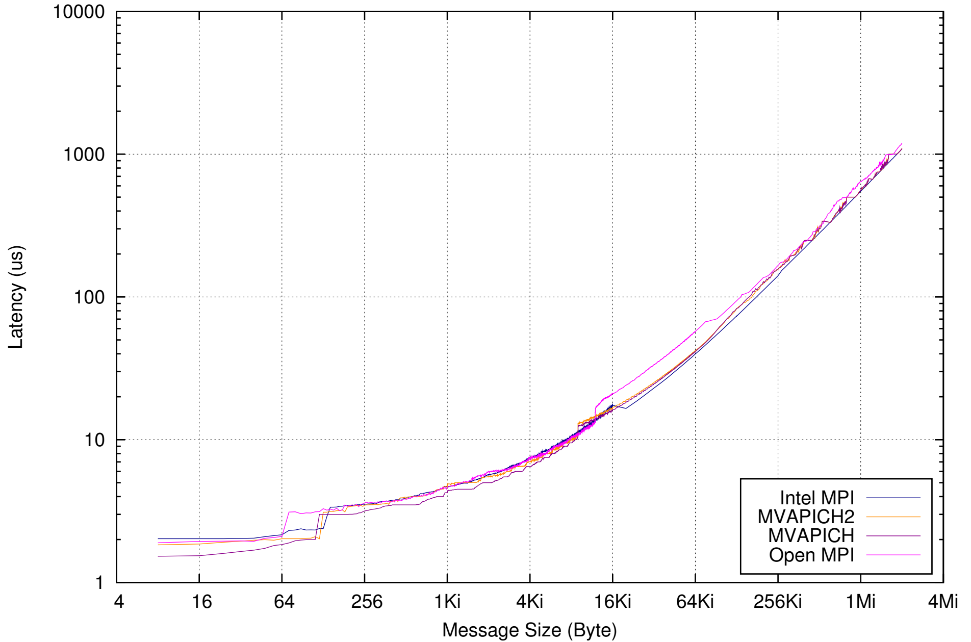
Latency comparison Zuse-Cluster, MPI implementations
