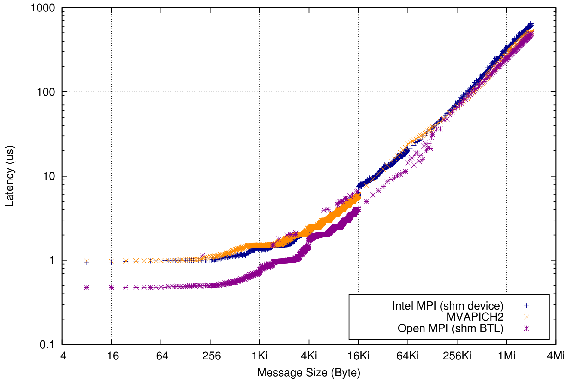
Intra Node communication Zuse Cluster, latency comparison
