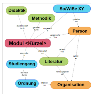
Abb. 1: Nav.-Graph – Basis
